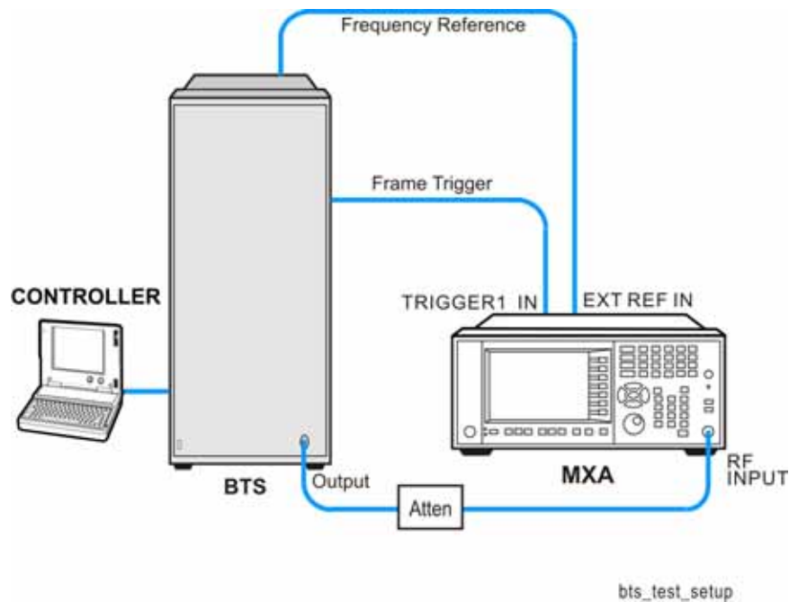
Figure 1-5 Adjacent Channel Power Measurement System
