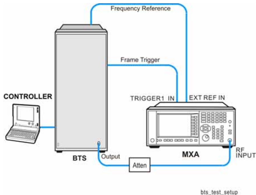
Figure 1-30 Code Domain Power Measurement System—RF
