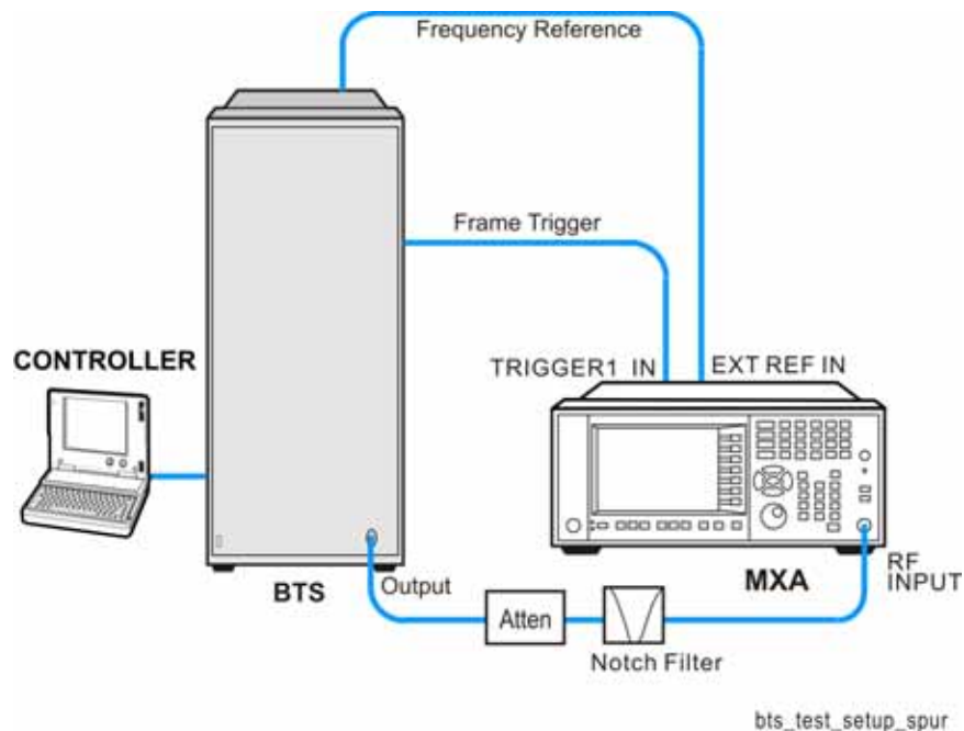
Figure 1-17 Spurious Emission Measurement System
