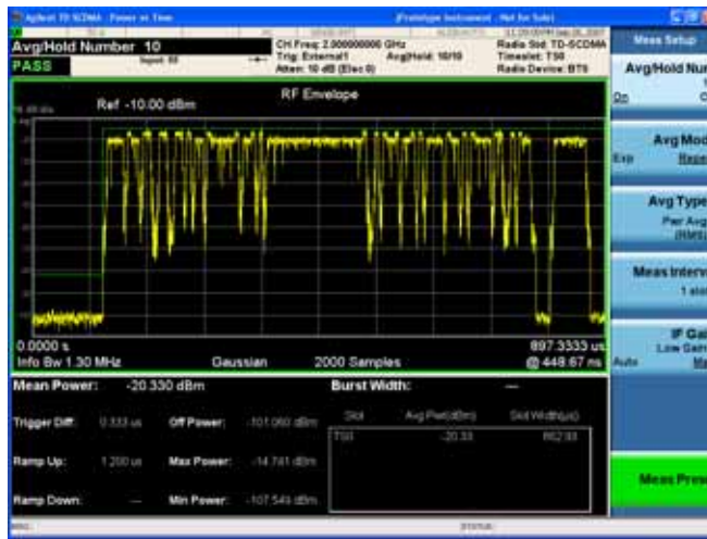
Figure 1-10 Power vs Time - Single-Slot View (Default)
