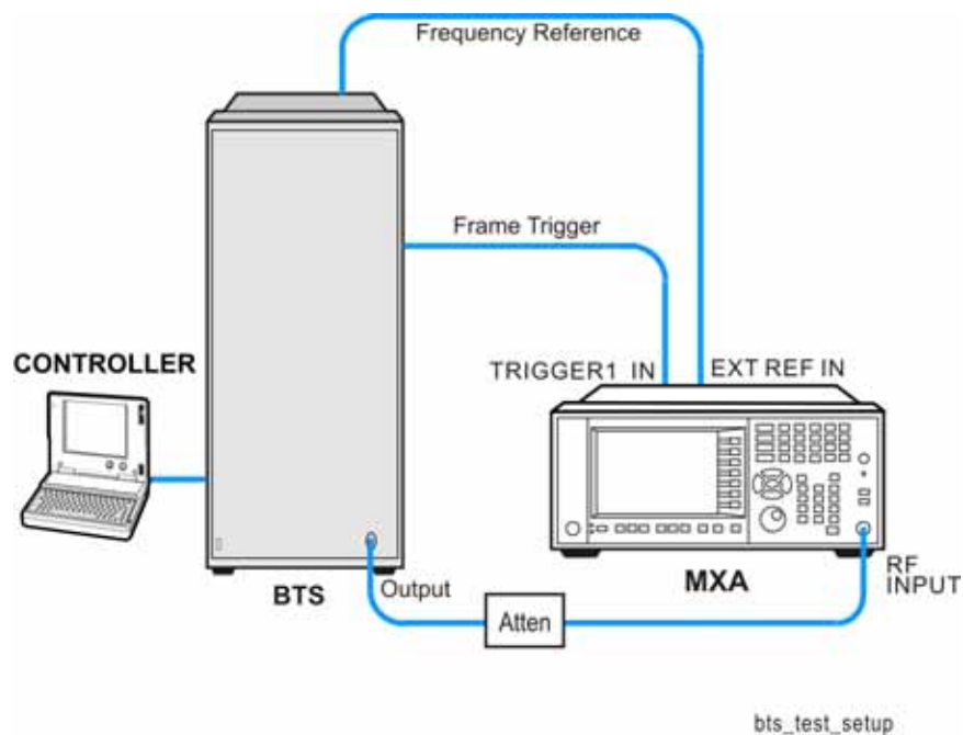
Figure 1-1 Transmit Power Measurement System
