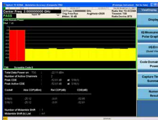
Figure 1-27 Modulation Accuracy - Code Domain Power View
