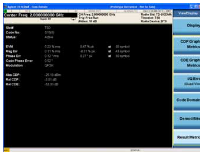
Figure 1-37 Code Domain Measurement - Result Metrics View
