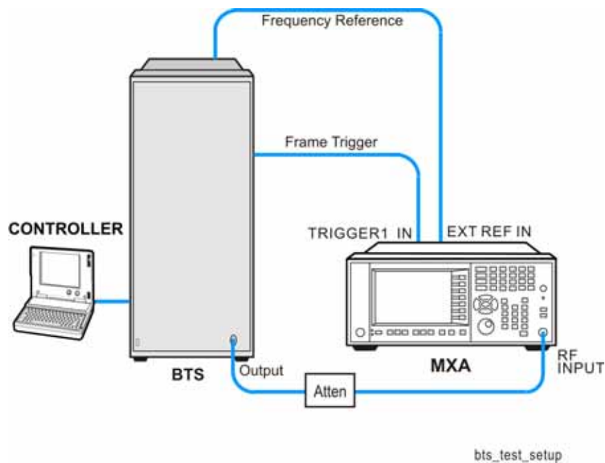
Figure 1-38 Transmit Power Measurement System
