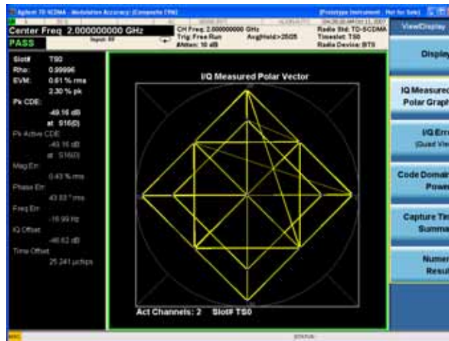
Figure 1-26 Modulation Accuracy - I/Q Measured Polar Graph View (Default)
