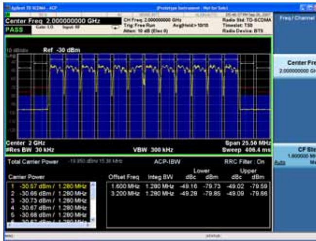
ACP - Multiple Carriers
