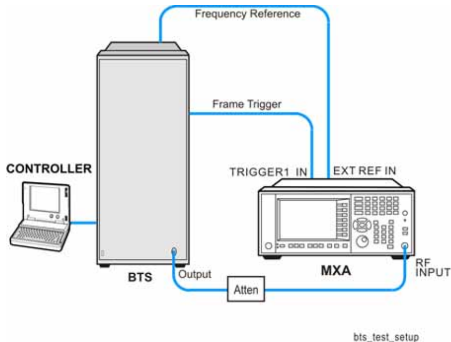
Figure 1-21 Power Statistics (CCDF) Measurement System
