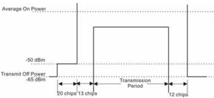
Figure 3-7 Power vs Time Measurement MS Mask
