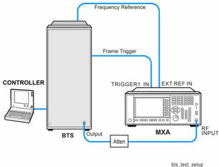
Figure 1-24 Modulation Accuracy Measurement System
