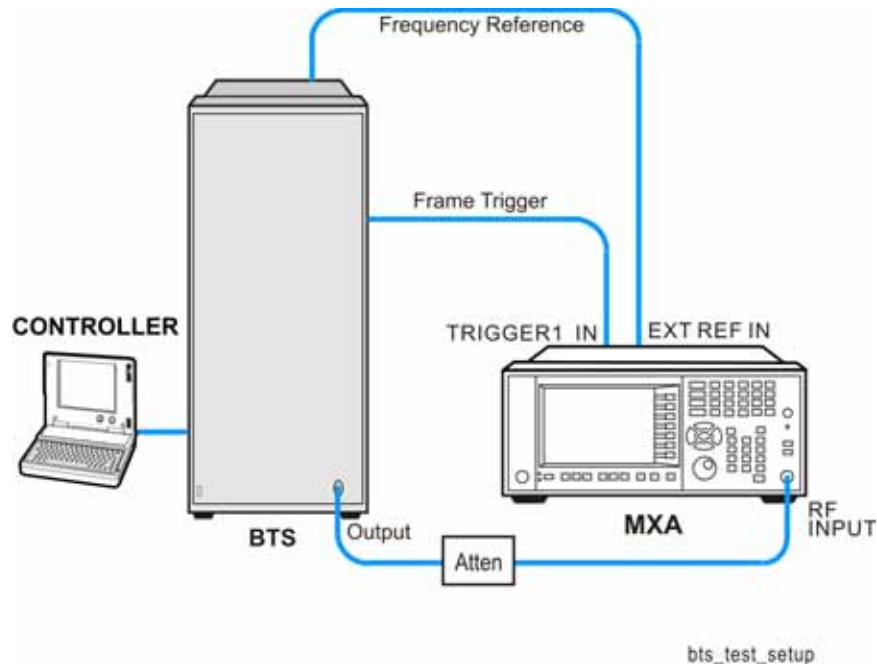
Figure 1-42 Transmit Power Measurement System
