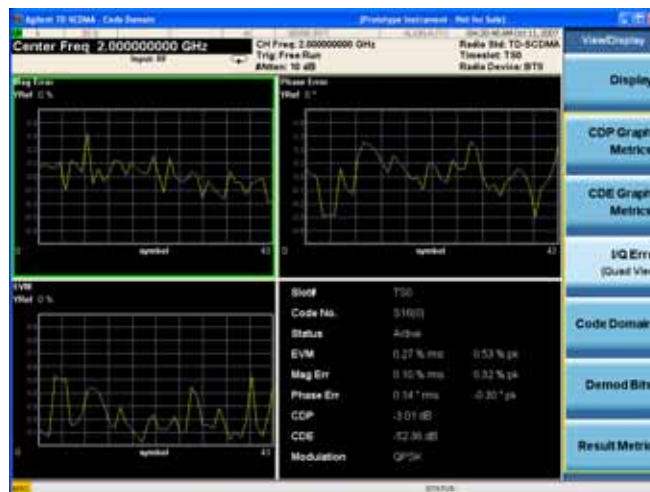
Code Domain Measurement Result - I/Q Error Quad View
