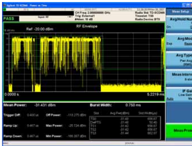
Figure 1-11 Power vs Time - Multi-Slot View (Meas Interval = 9)
